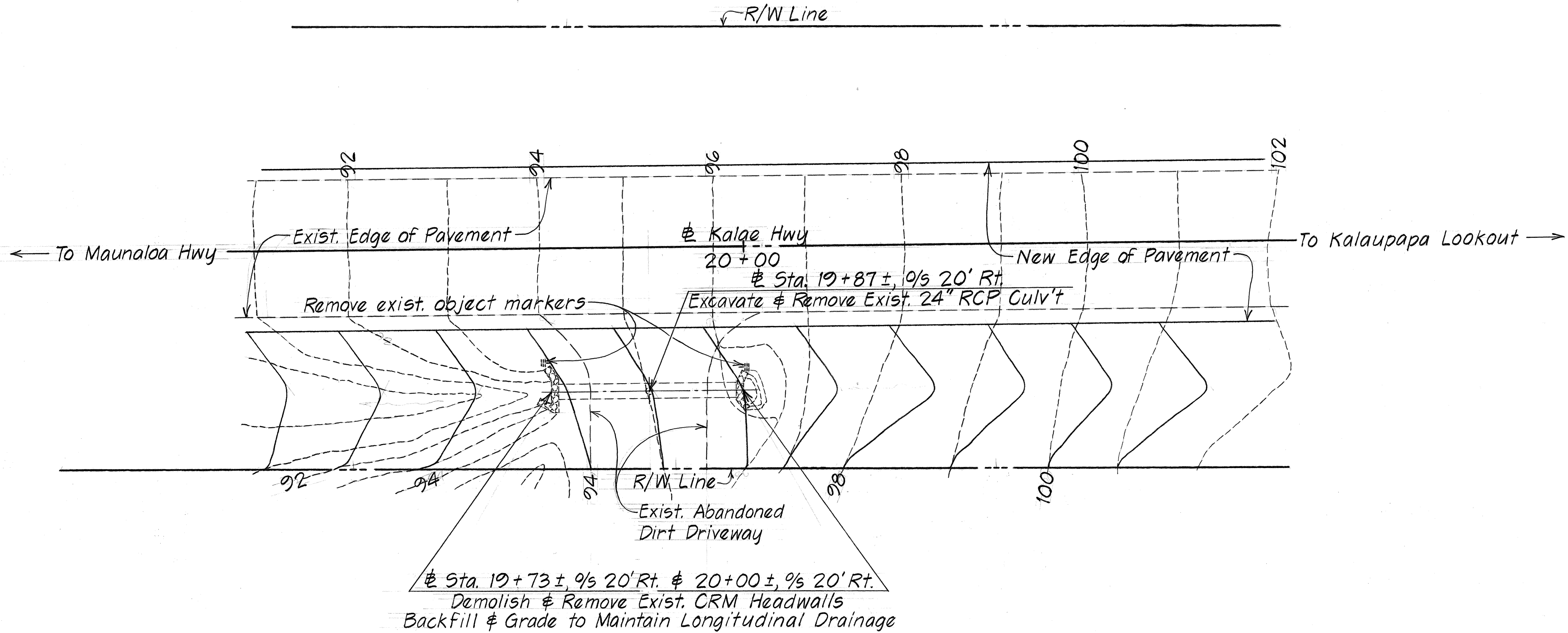
PLAN - STA. 19 + 87 KALAE HWY. Scale : 1" = 10'
